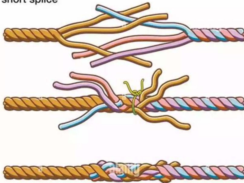
short splice
